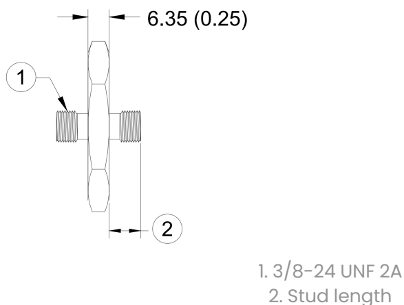
Figure 1: Hex Plate Stud for "A" Options 02, 03, 05, 17, 18, and 23.
