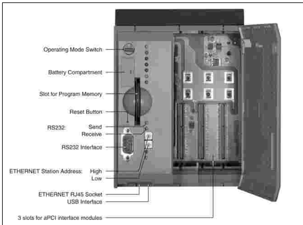
Figure 58: CP382 operational and connection elements
