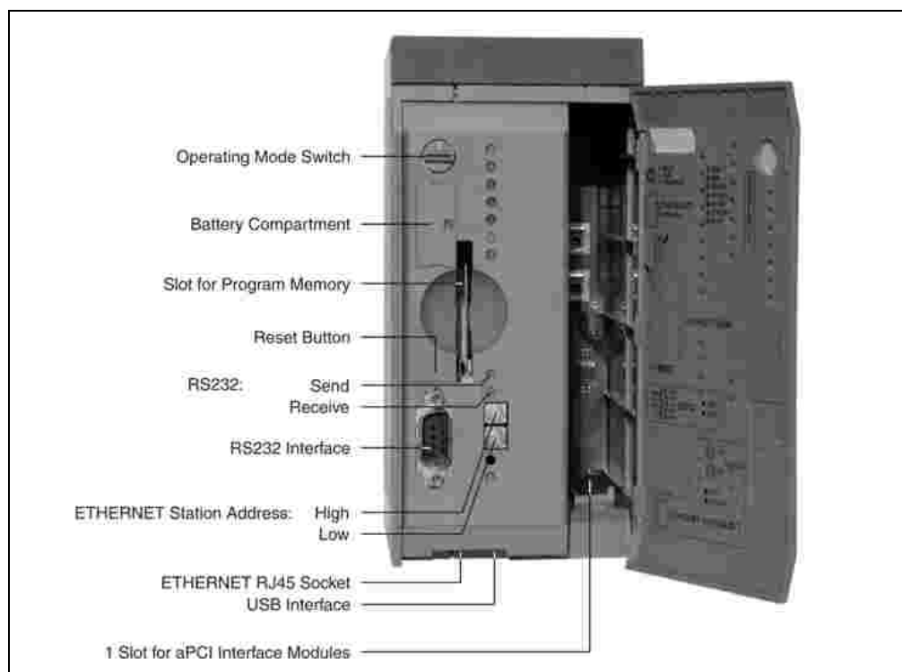
Figure 57: CP340, CP360 and CP380 operational and connection elements
