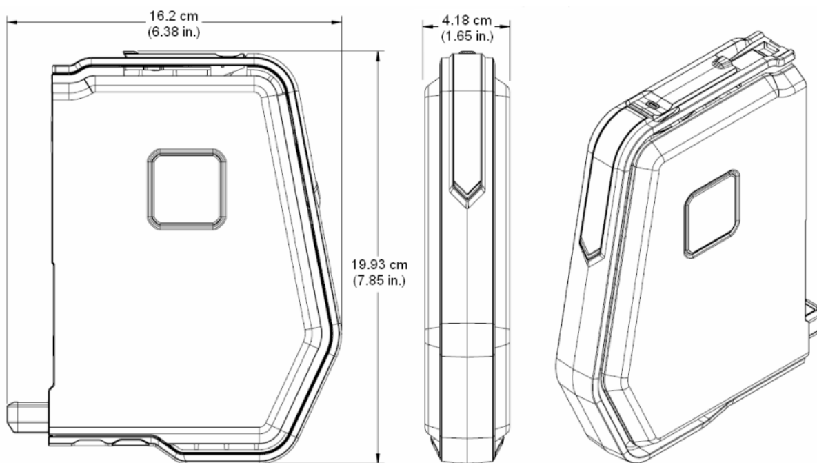
DeltaV SQ controller hardware dimensions.
