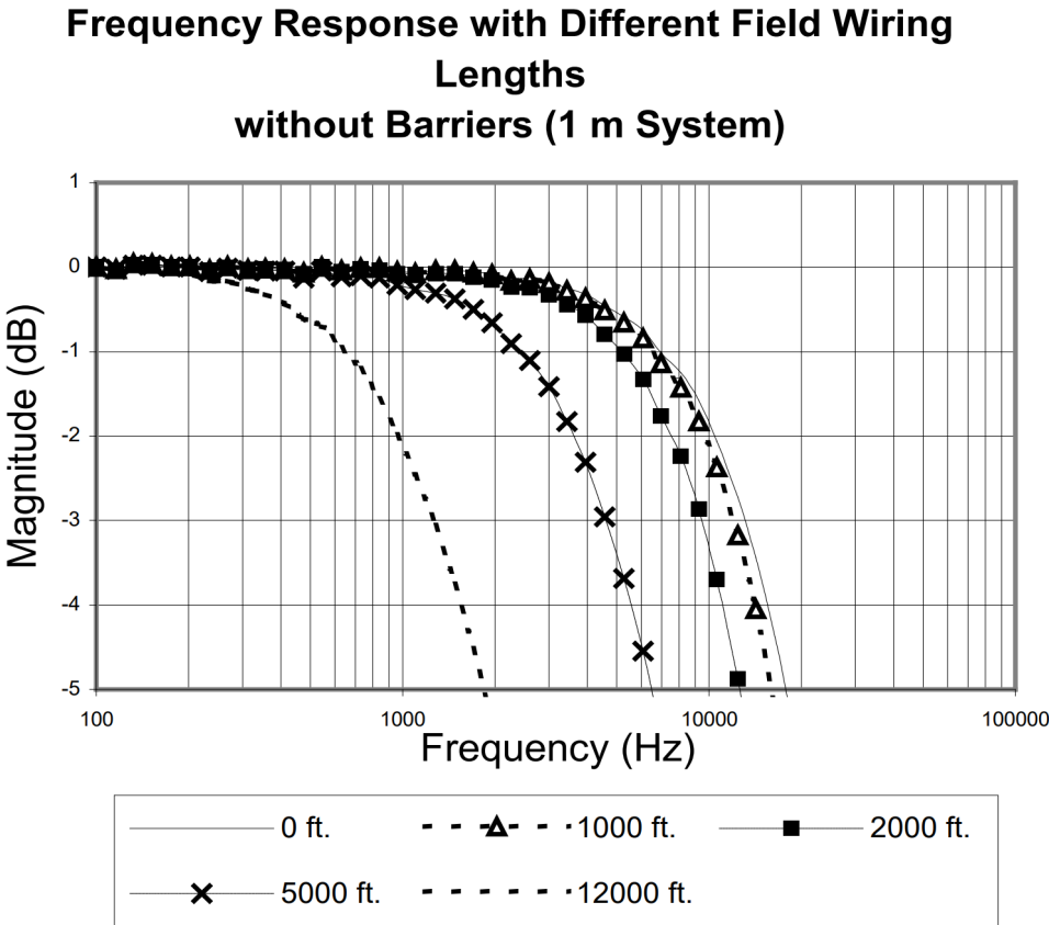
Figure 1: Frequency Response with Different Field Wiring Lengths without Barriers (1 m System)
