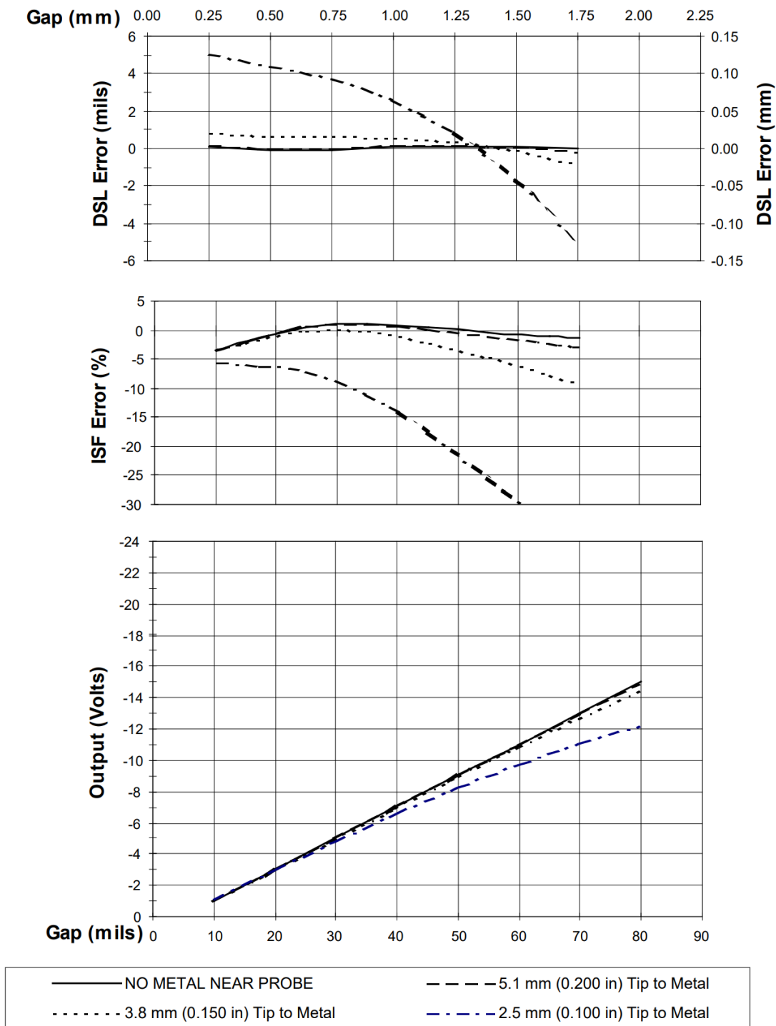
Figure 11: Effect of Rear Surface Clearance (4140 Material)
