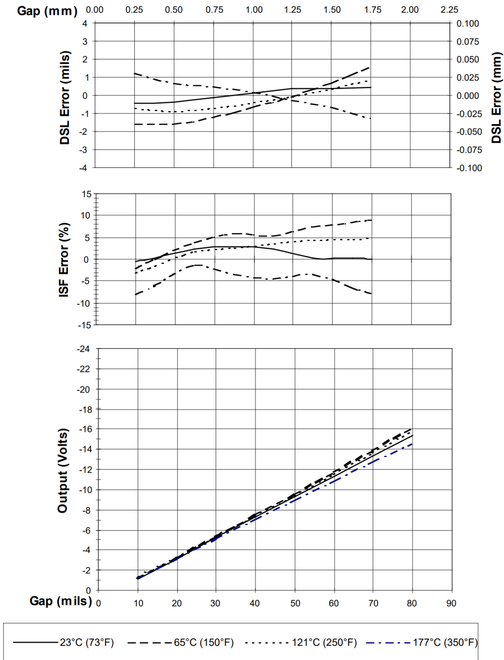
Figure 4: Typical 3300 NSv Probe + 1 m Cable @ High Temperature (Proximity Sensor + 4 m of Extension Cable @ 25°C)
