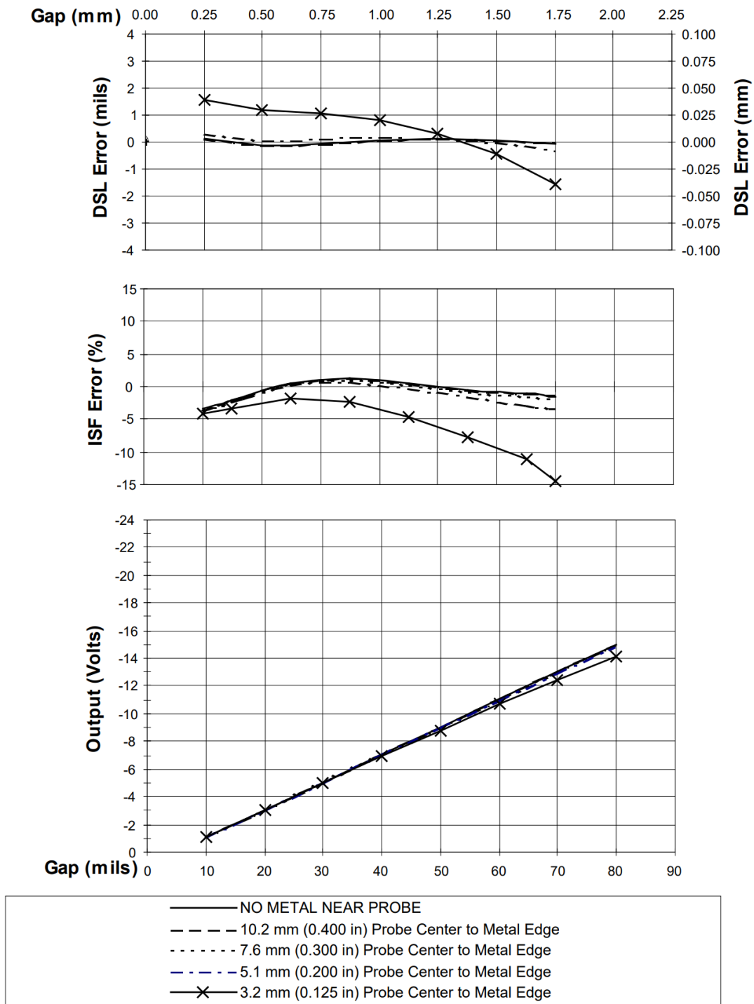
Figure 10: Effect of Flat Surface Side Clearance (4140 Material)
