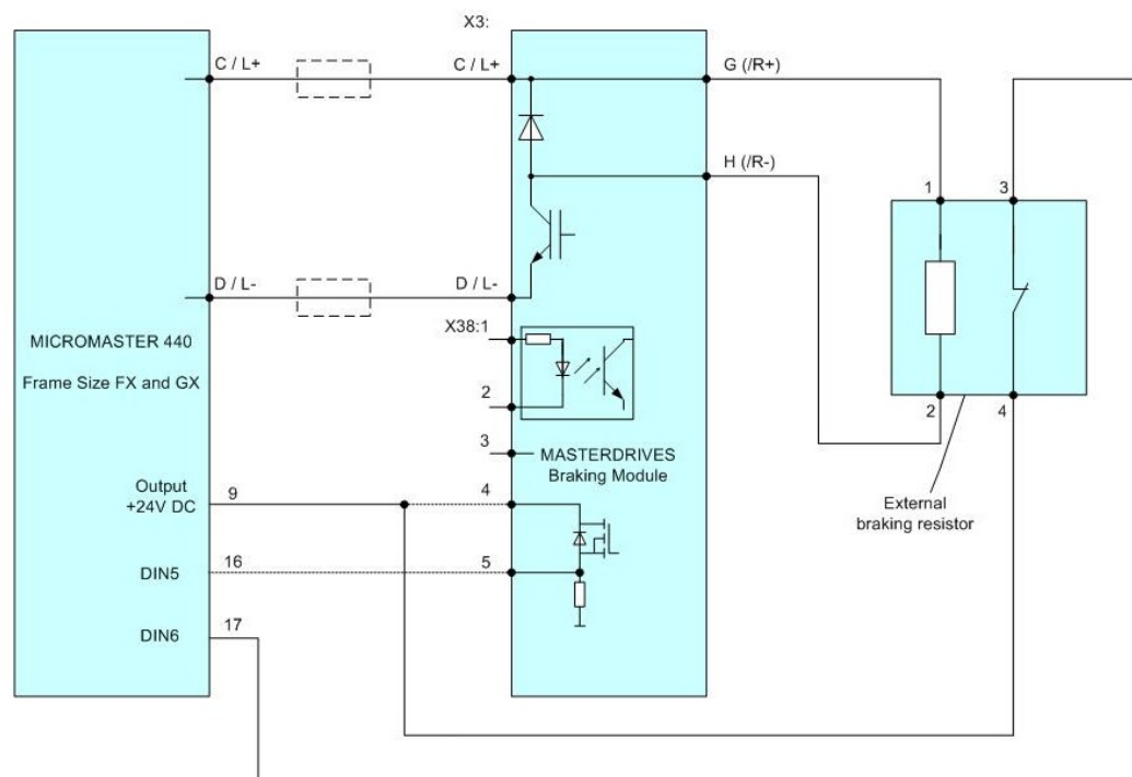
Figure 3-1 Connecting the braking module to drive inverters MM440, FX and GX
