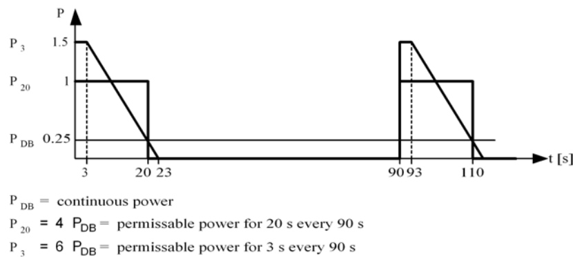
Figure 1-1 Load diagram of the braking module with external braking resistor
