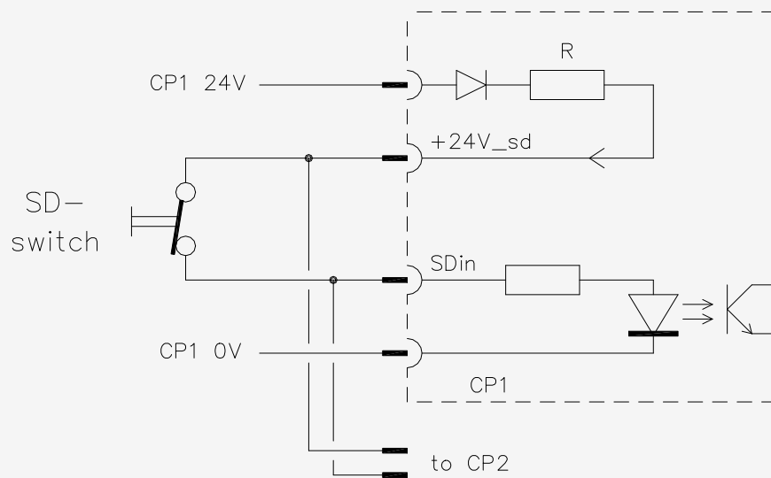
Figure 7-4: SD input schematic
