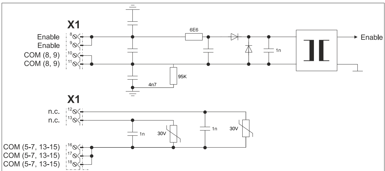
Figure 6: Enable
