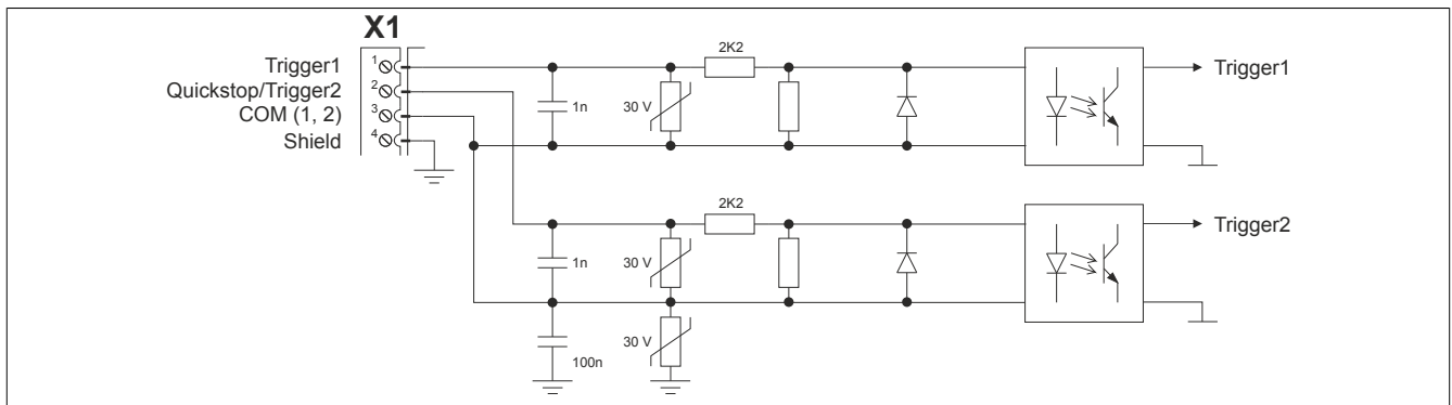
Figure 4: Trigger
