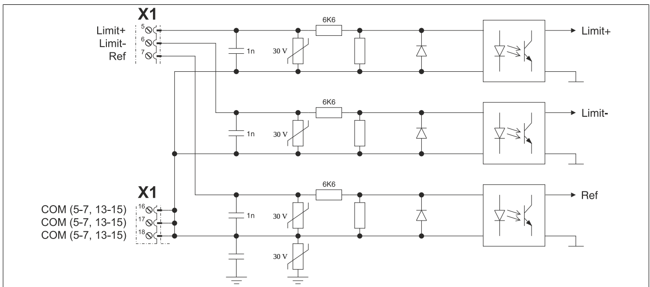
Figure 5: Limit
