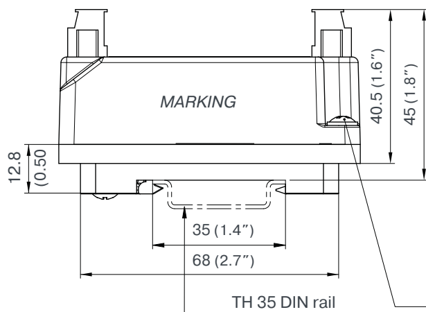
Side and end views with DIN-rail mounting adaptor (ordering option code G2)
