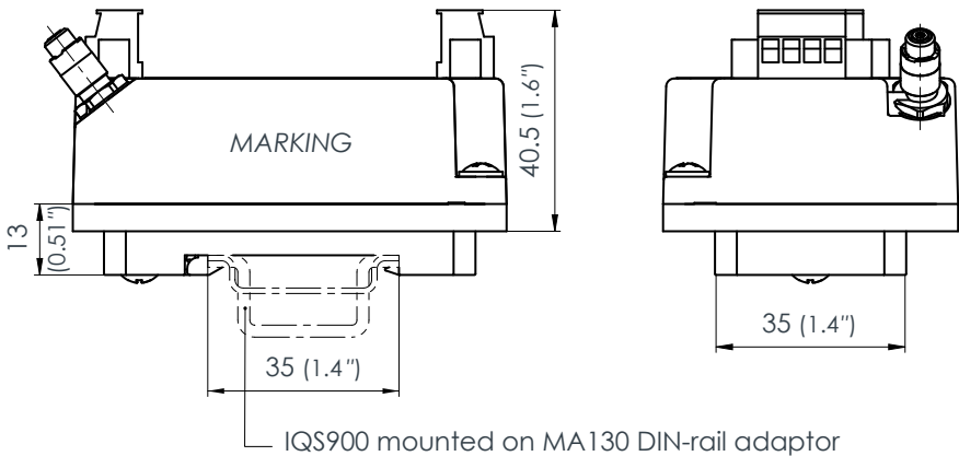
IQS900 mounted on MA130 DIN-rail adaptor
