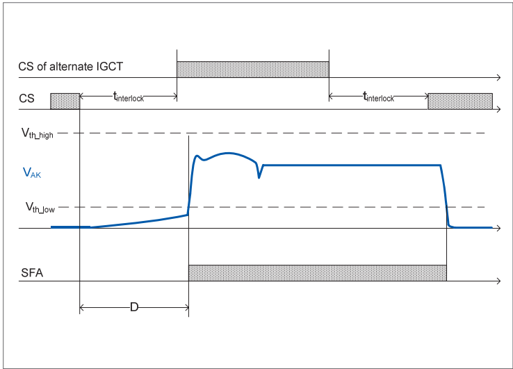
17 Turning off low current
