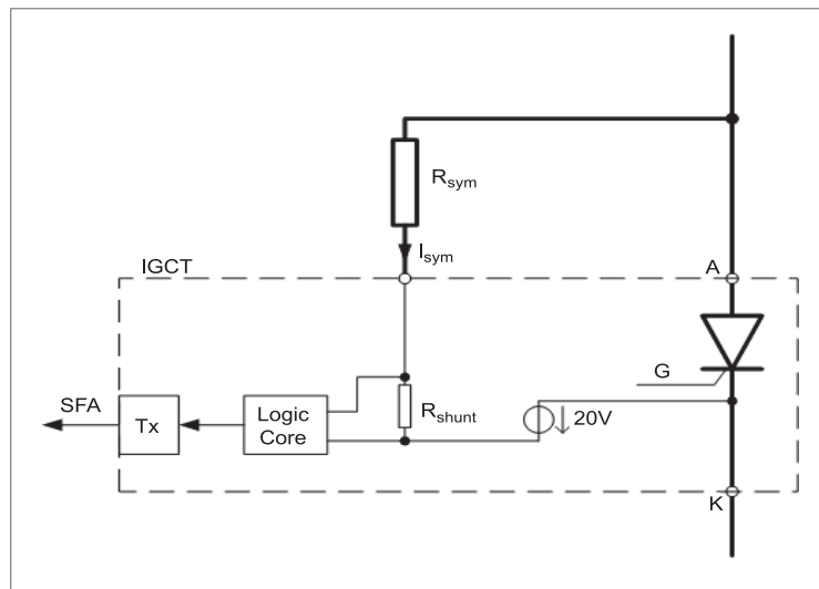
14 Principle of anode voltage monitoring
