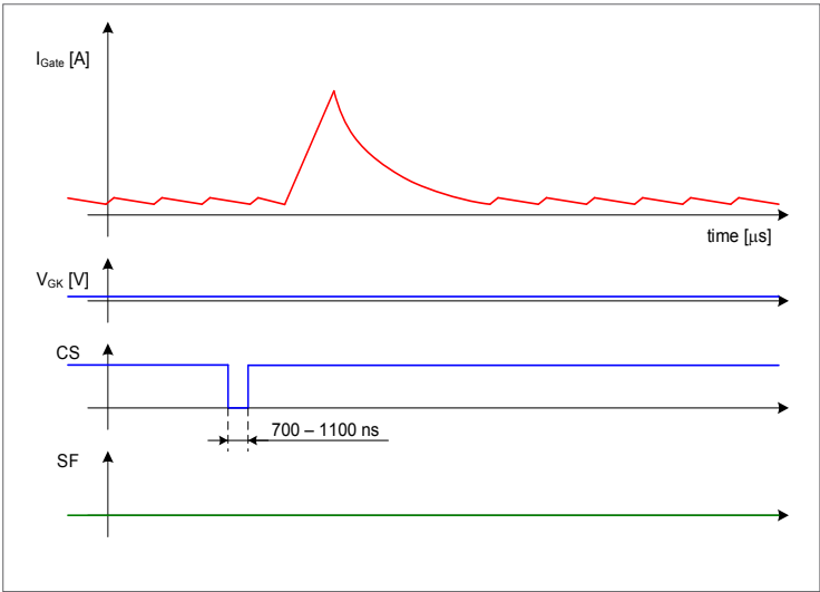
12 External re-trigger (measurement)
