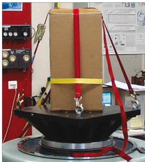
22 Vibration test with IGBTs wrapped in transport box
