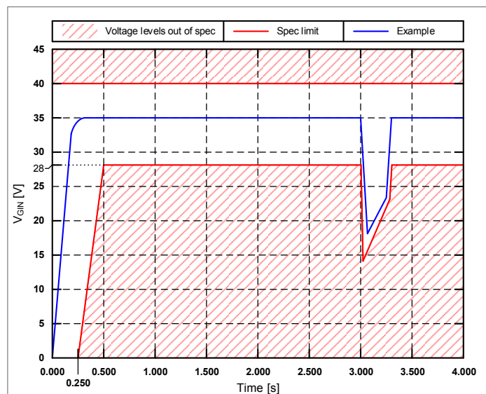
09 Gate unit start up
