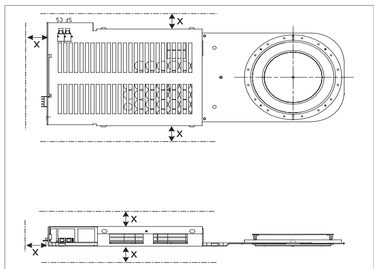
19 Distance between gate unit and parts with high di/dt
