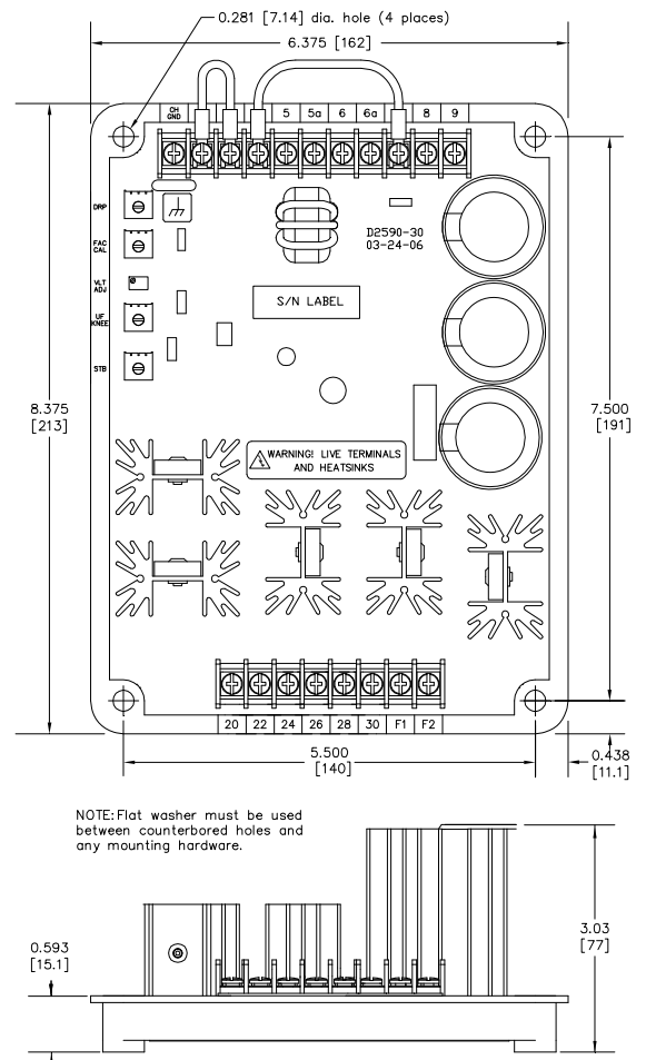
Figure 5. Outline Drawing
