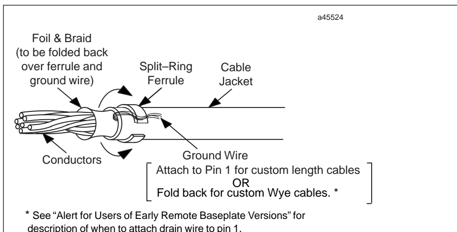
Figure 10-16. How to use Split-Ring Ferrules for Foil and Braided Cable Shield
