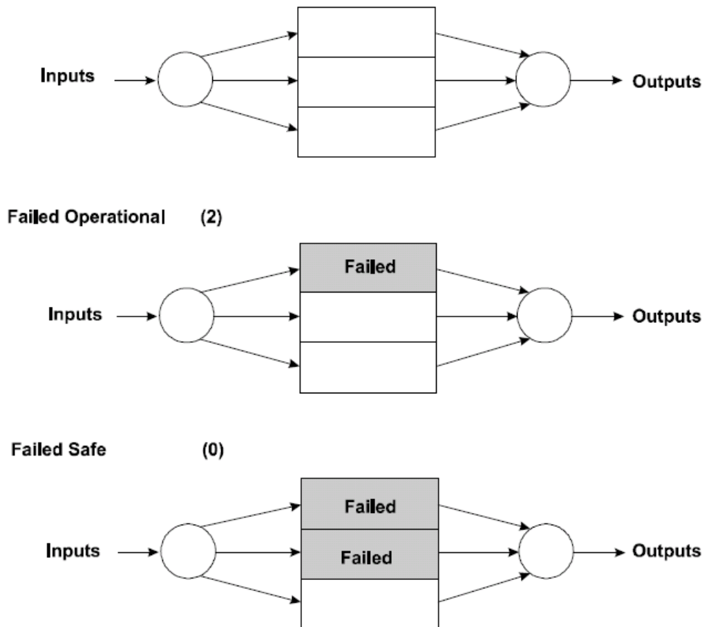
Figure 3-3: 3-2-0 Operation
