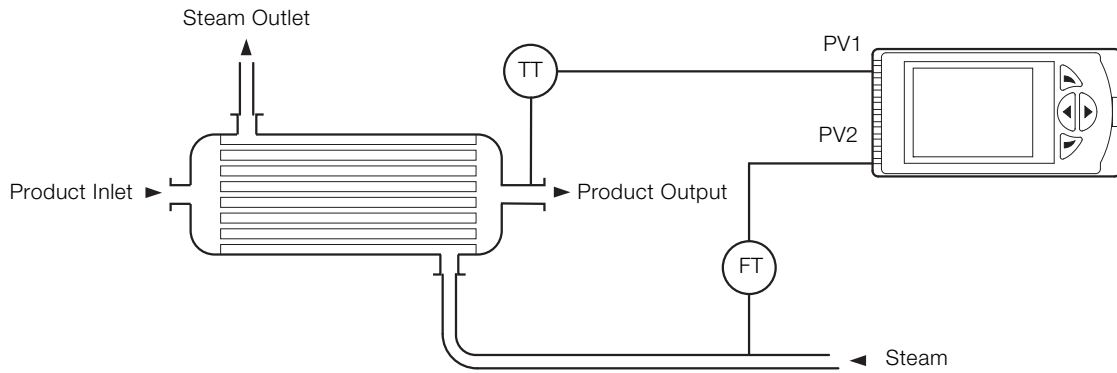
Fig. 15: Dual indication
