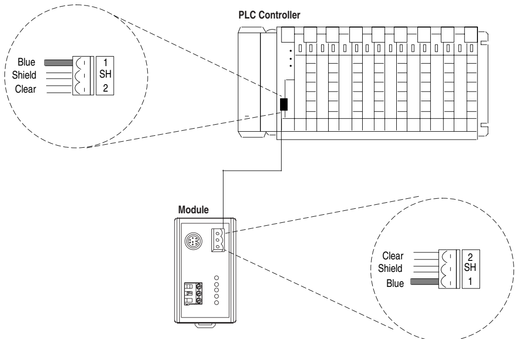
Figure 3.3 Connecting the Remote I/O Cable
