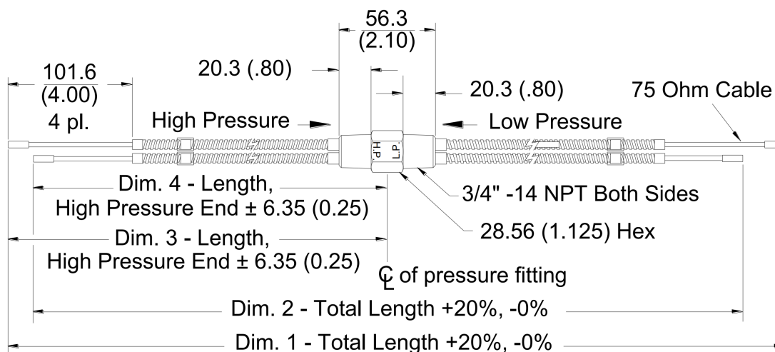
Figure 4: Part Number 330762 Dual Feedthrough, 3300 XL 11mm System
